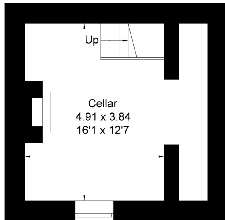
Cellar
