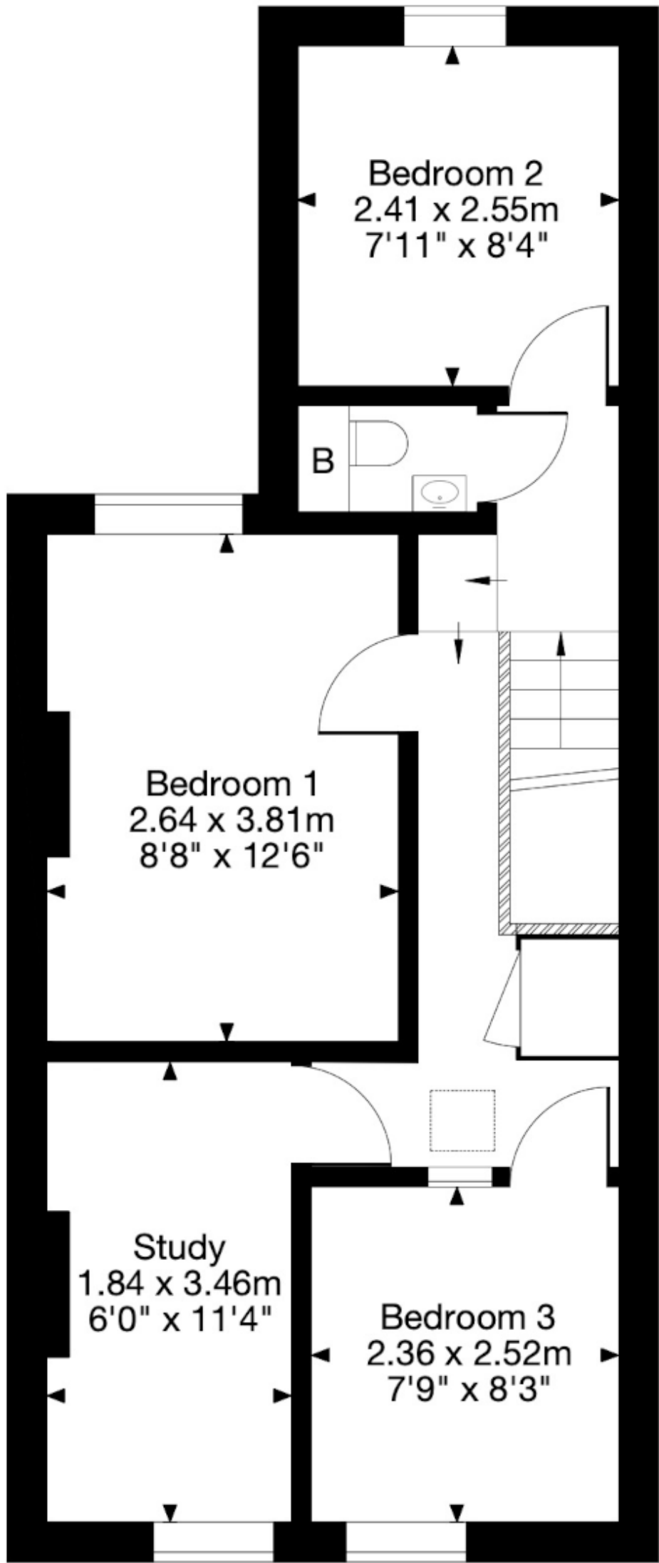
First Floor
